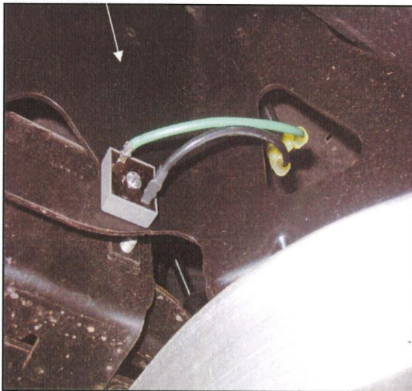
Voltage Limiter
